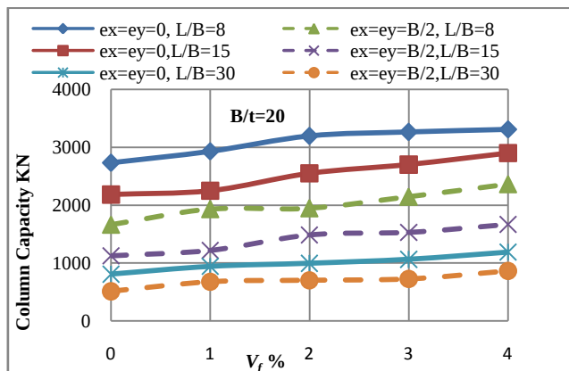
Figure 7 Column capacity versus V_f\% for different L/B ratios
